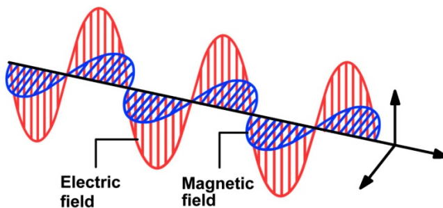
Electromagnetic Waves
